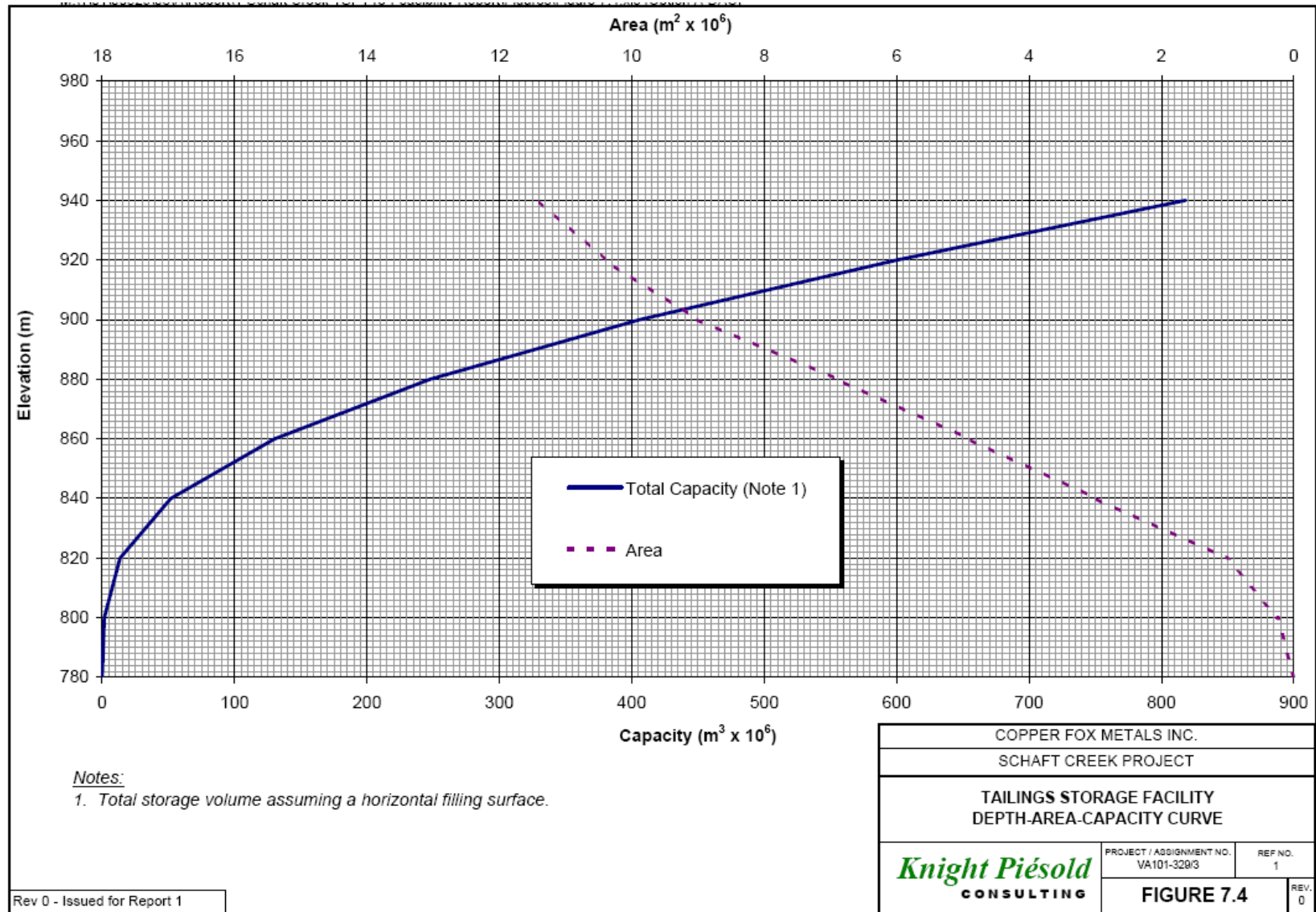
Figure 25.36 Depth-Area-Capacity Curve
