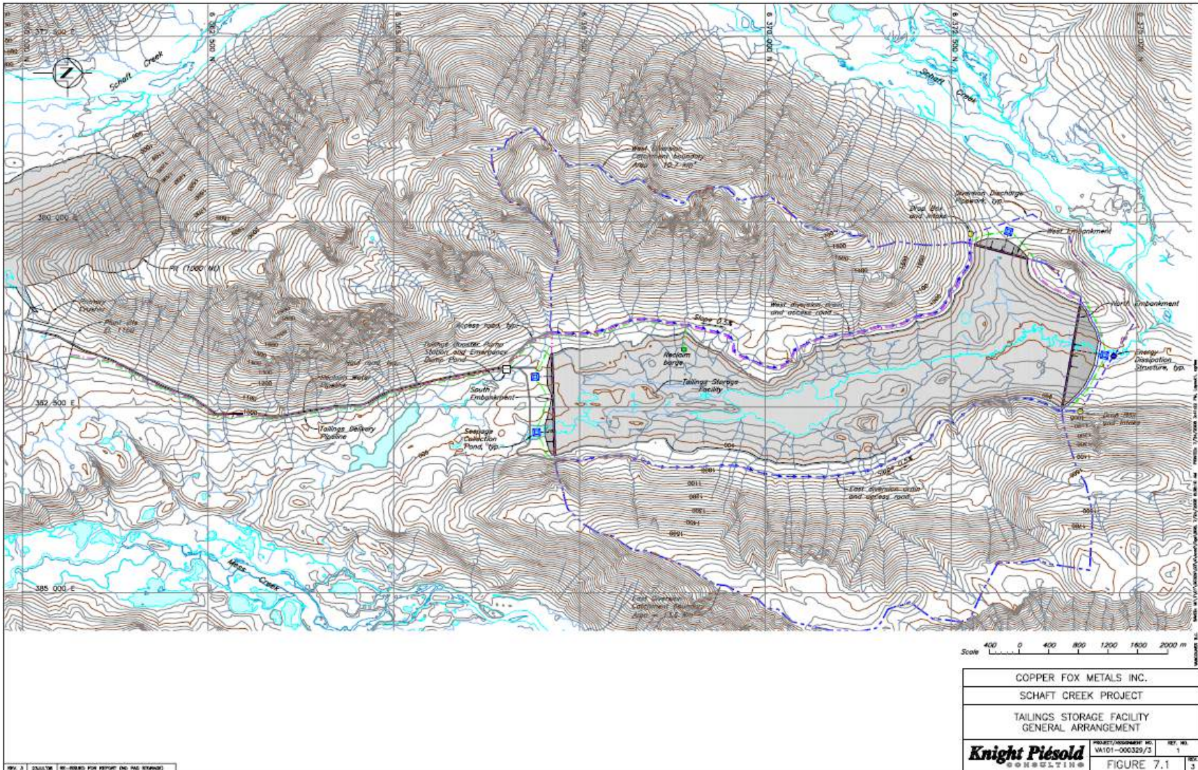
Figure 25.33 General Arrangement
