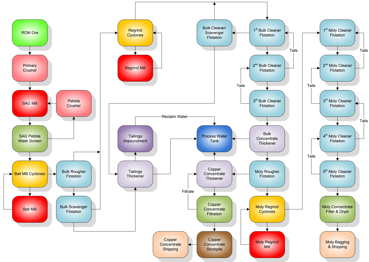
Figure 18.9 Block Flow Diagram
