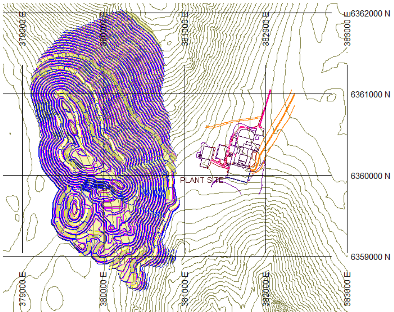
Figure 25.4 Plan View of the Ultimate Pit P651i
