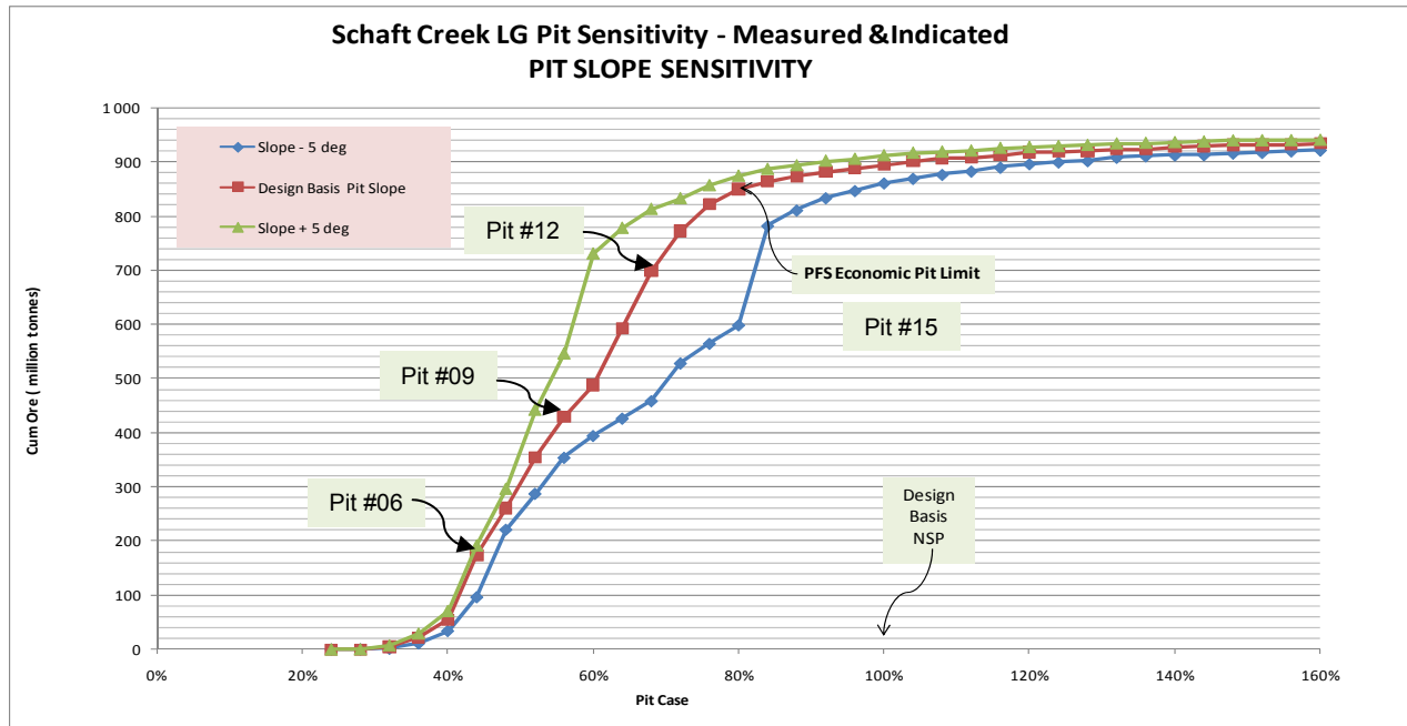
Figure 25.1 Economic Pit Limit Overall Pit Slope Sensitivity
