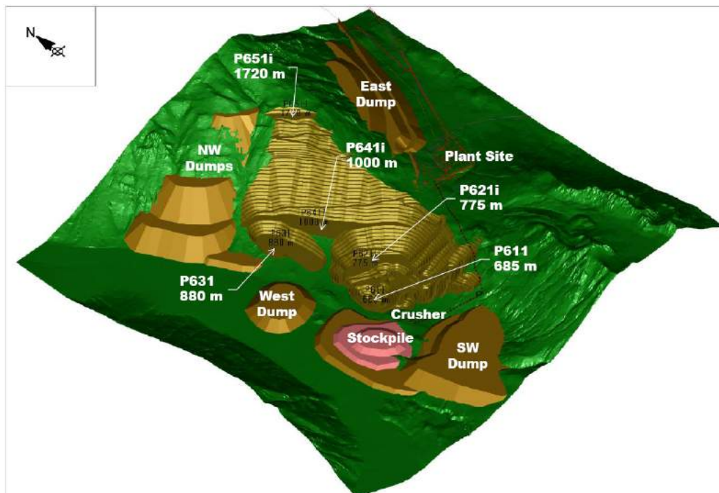
Figure 25.19 End of Year 10 Orthographic View from the SW
