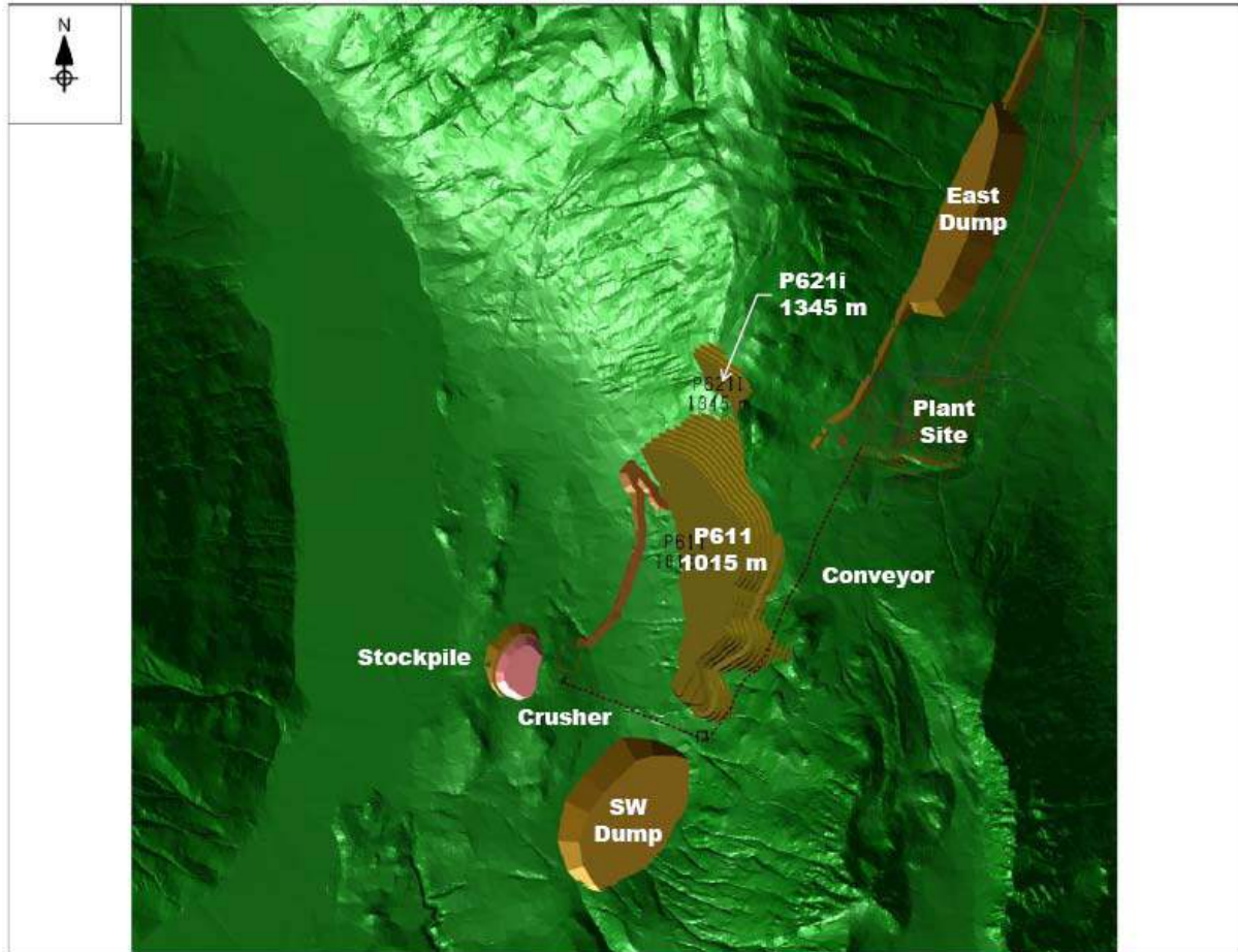
Figure 25.12 End of Year 1 Plan View
