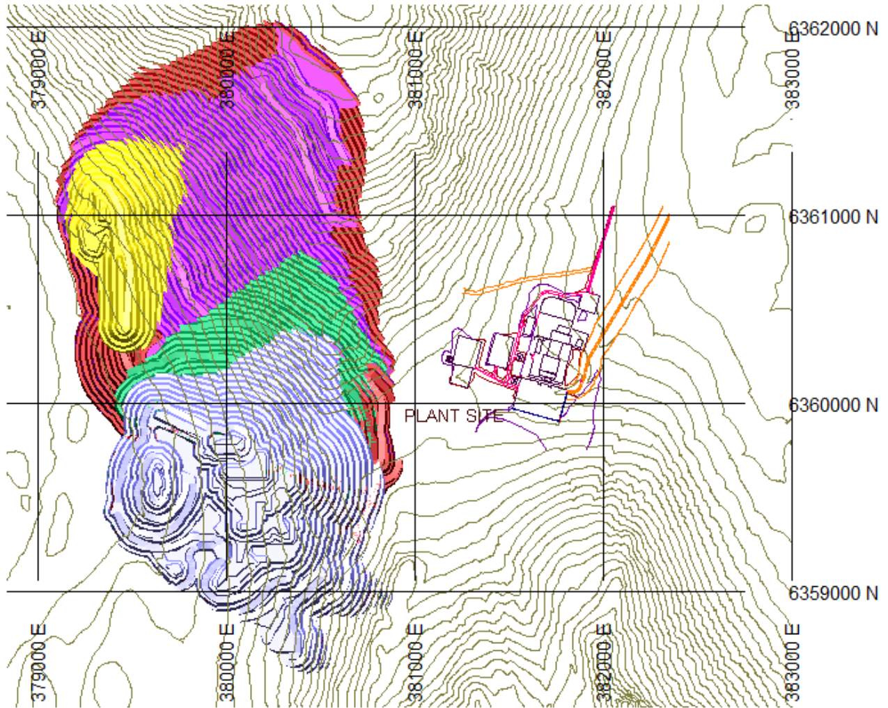
Figure 25.5 Plan View of All Designed Pit Phases
